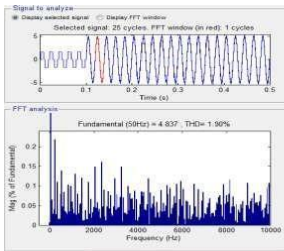
Figure 17: FFT Analysis of Source Current of Proposed 4-Leg with VSI with Balanced Non Linear Load Condition
