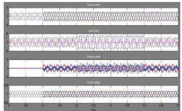
Figure 19: Source Current, Load Current, Inverter Injecting Current, Grid Voltage
