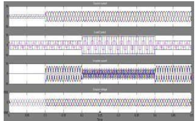
Figure 14: Source Current, Load Current, Inverter Injecting Current, Grid Voltage
