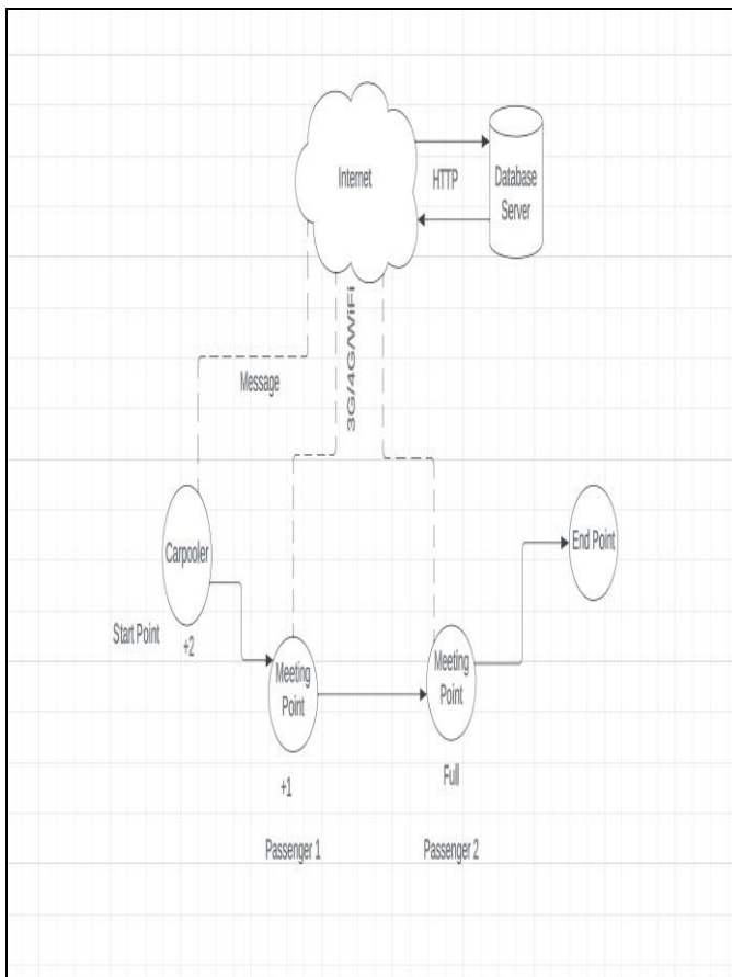
Fig 1- System Architecture
