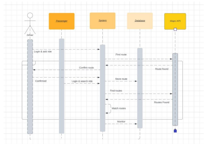
Fig 1- Sequence Diagram
