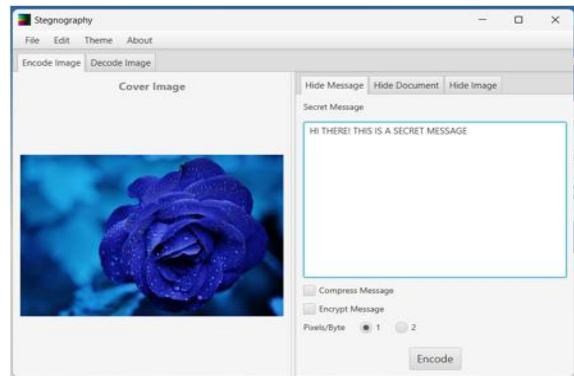
Fig -3: Hiding of secret data
