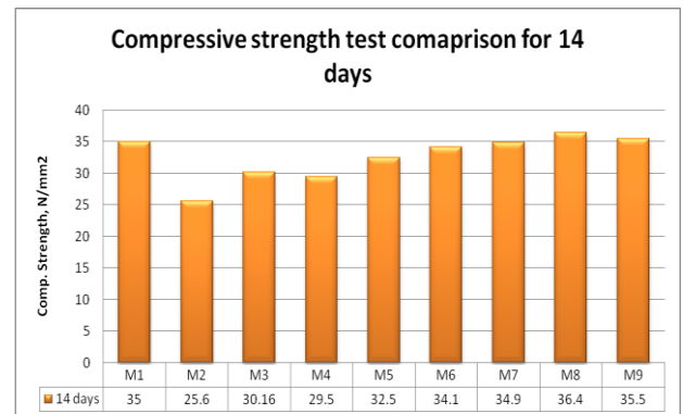
Fig. 3 Compressive strength comparison for 14 days
