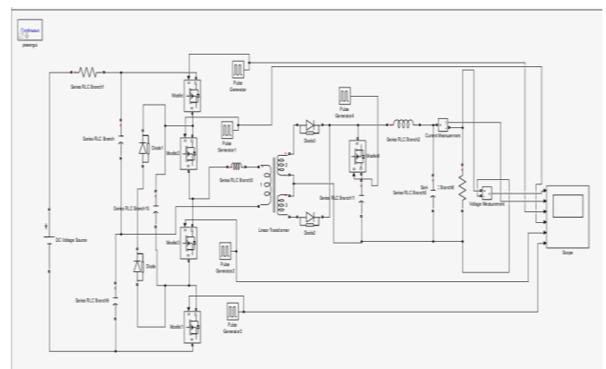
Fig.2. Simulink Model of Three level Buck Converter with ZVS Method
