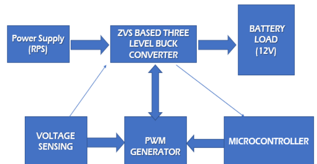
Fig.1. The Proposed System Operation Sequence
