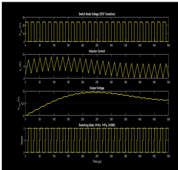
Fig.3. Simulink Model of Three level Buck Converter using ZVS Method – Output Waveform
