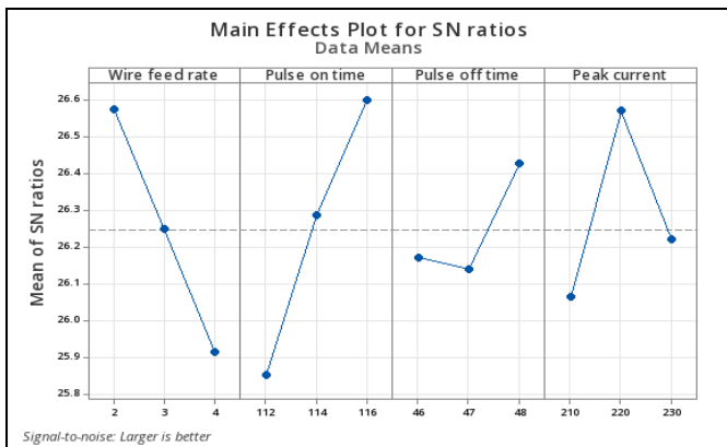
Chart -2: Main Effects Plot For S/N Ratios
