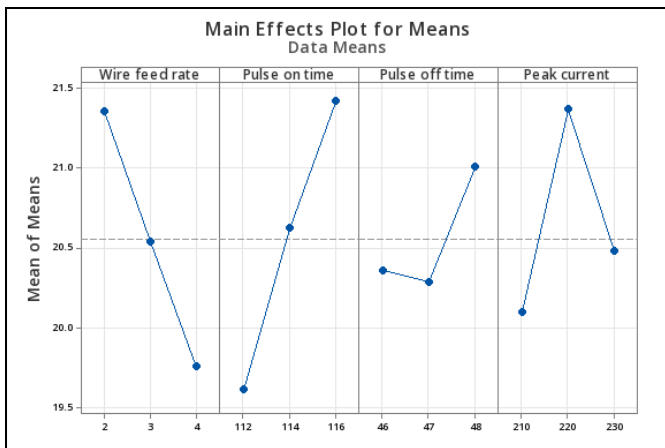
Chart -1: Main Effects Plot For Means
