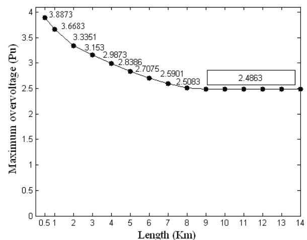
Fig -2: Maximum overvoltage as function of cable length.
