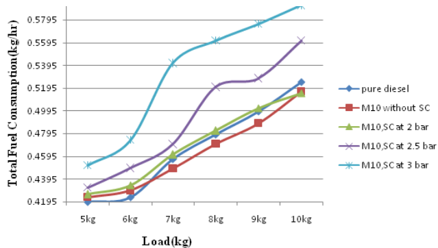
Variation of Total Fuel Consumption with loads for M10 blend
