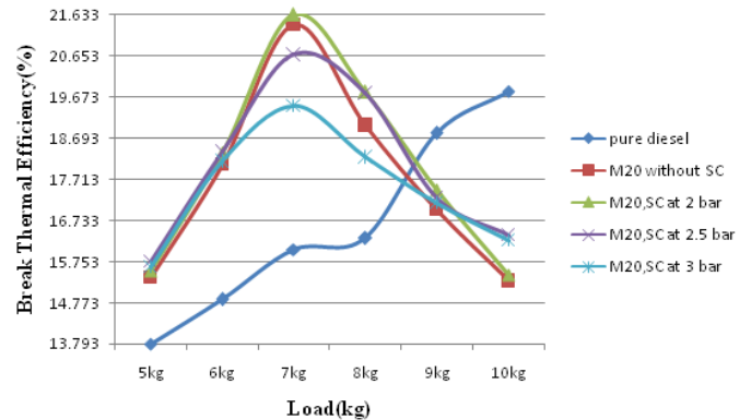
Variation of Break Thermal Efficiency with loads for M20 blend
