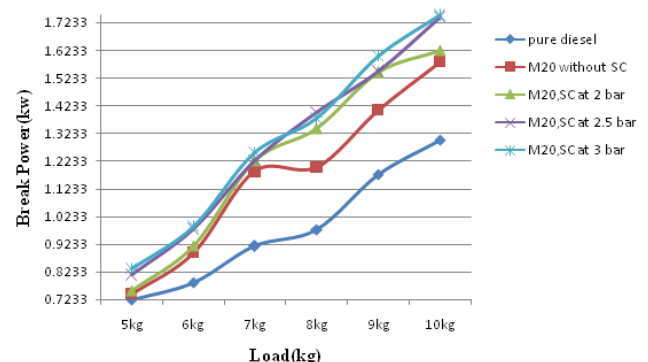
Variation of break power with loads for M20 blend
