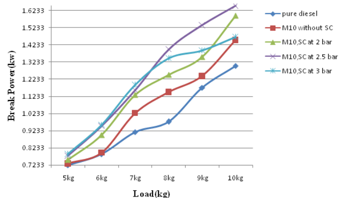
Variation of break power with loads for M10 blend
