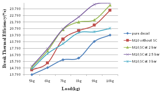
Variation of Break Thermal Efficiency with loads for M10 blend
