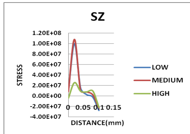
Graph 5.3.4.3 Effect of speed on stress along Z direction
