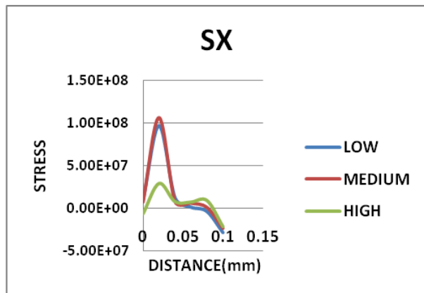
Graph 5.3.4.1 Effect of speed on stress along X direction
