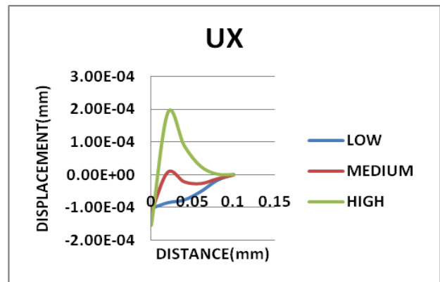
Graph 5.2.1.1 Effect of heat input on displacement along X direction
