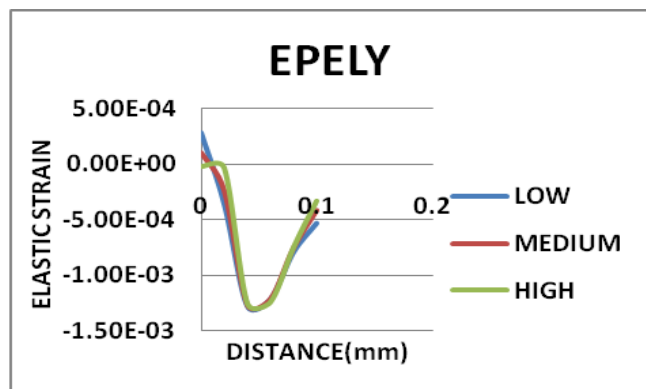
Graph 5.2.2.2 Effect of heat input on elastic strain along Y direction
