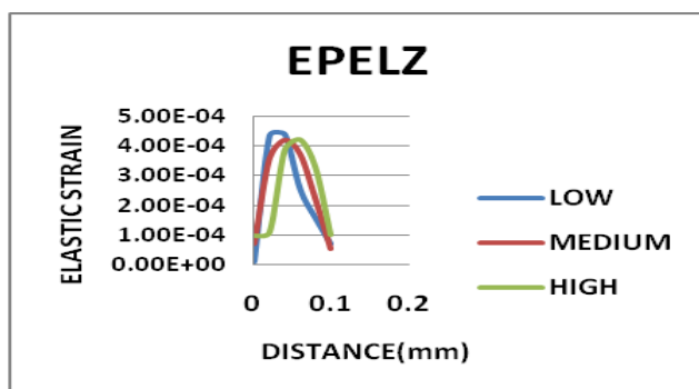
Graph 5.3.2.3 Effect of speed on elastic strain along Z direction
