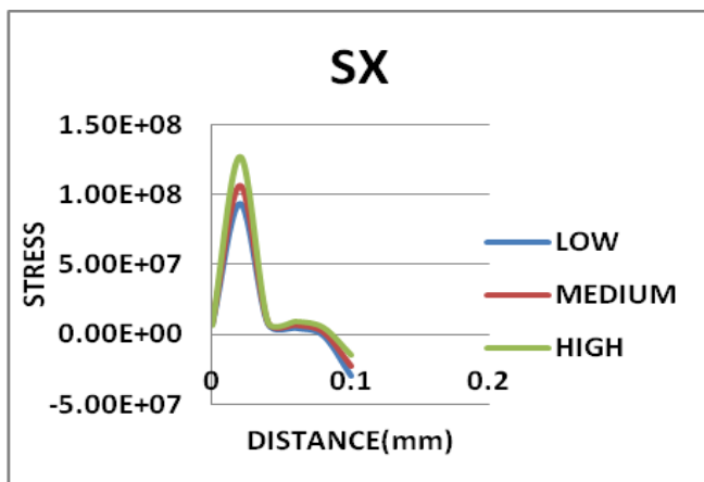
Graph 5.2.4.1 Effect of heat input on stress along X direction
