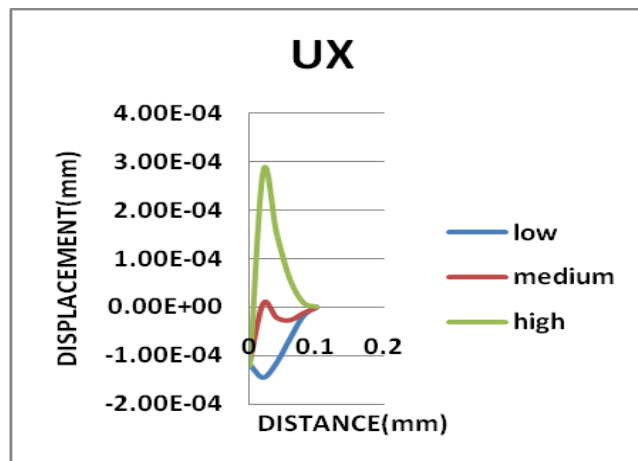
Graph 5.3.1.1 Effect of speed on displacement along X direction
