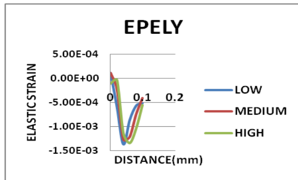
Graph 5.3.2.2 Effect of speed on elastic strain along Y direction
