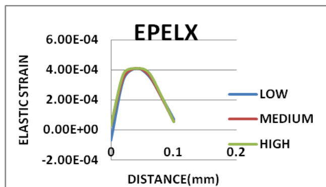
Graph 5.2.2.1 Effect of heat input on elastic strain along X direction
