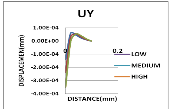
Graph 5.3.1.2 Effect of speed on displacement along Y direction
