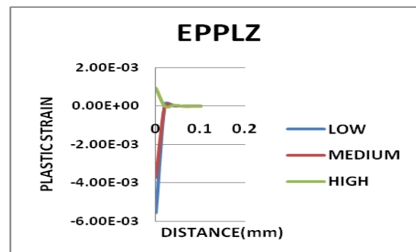
Graph 5.3.3.3 Effect of speed on plastic strain along Z direction
