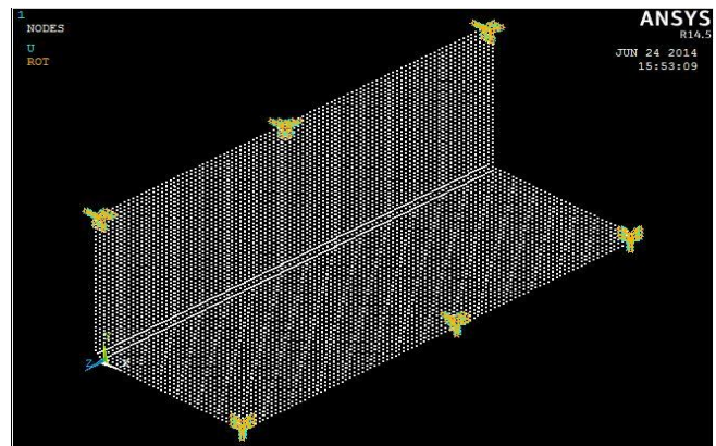
Figure 4.5.1 Boundary condition applied to the structural welded plates
