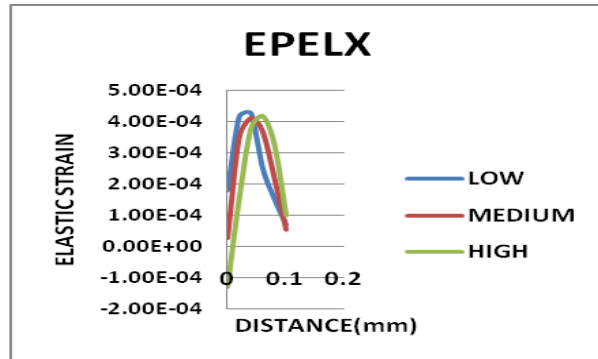
Graph 5.3.2.1 Effect of speed on elastic strain along X direction
