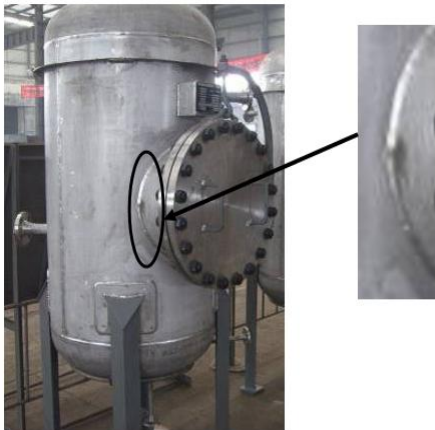
Figure 2.1.2 Welding joint used in pressure vessel
