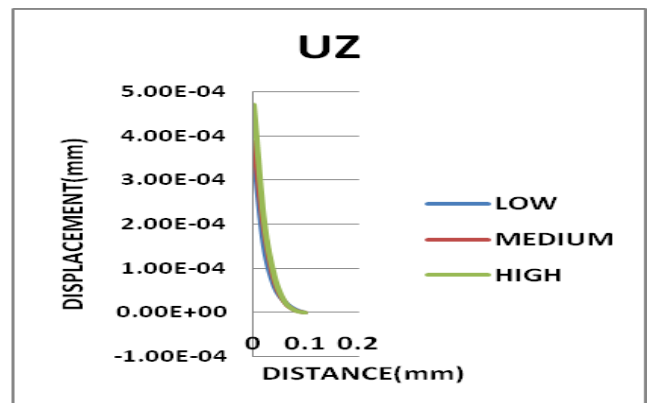
Graph 5.3.1.3 Effect of speed on displacement along Z direction
