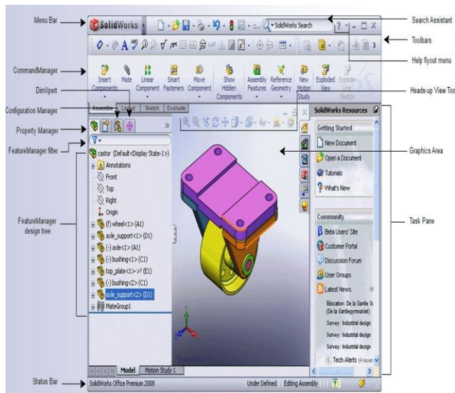
Figure 3.1.1 SolidWorks User Interface
