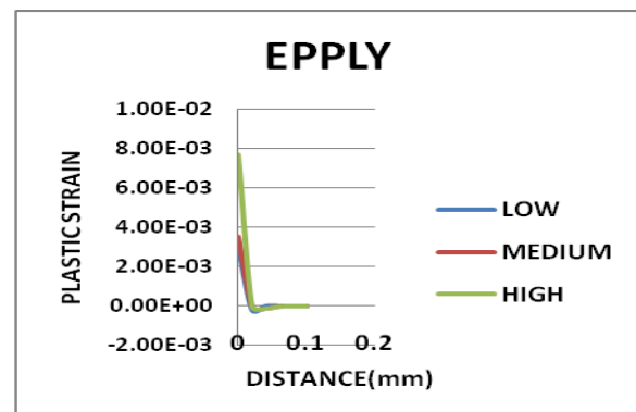
Graph 5.3.3.2 Effect of speed on plastic strain along Y direction
