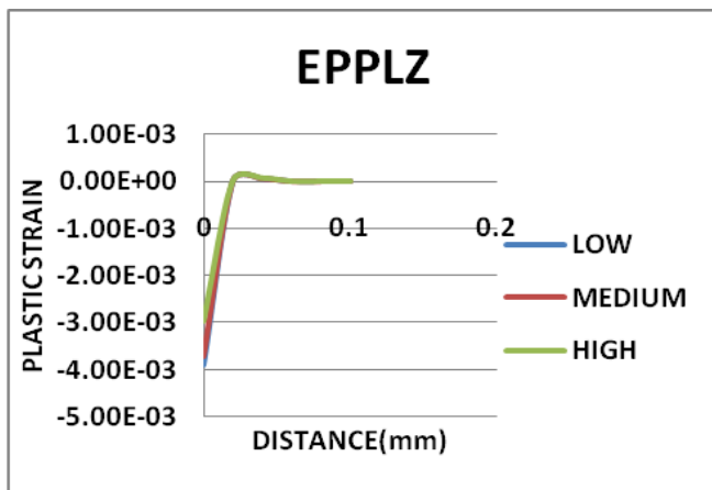
Graph 5.2.3.3 Effect of heat input on plastic strain along Z direction
