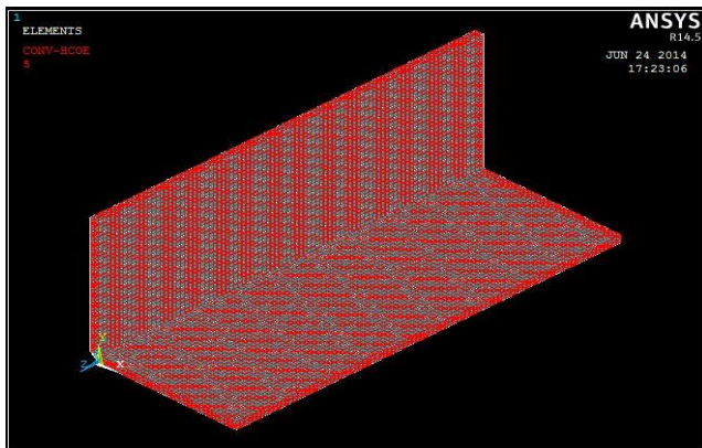
Figure 4.3.1 Boundary condition applied to the thermal welded plates
