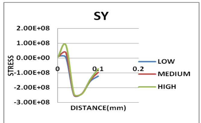
Graph 5.2.4.2 Effect of heat input on stress along Y direction
