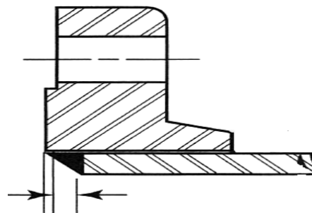
Figure 2.1.1 fillet Welding joint
