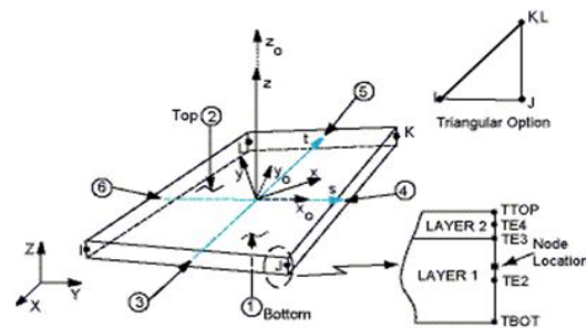
Figure 4.1.2 Geometry of Shell131 element
