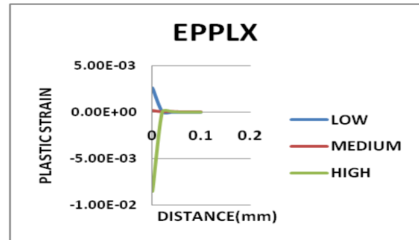
Graph 5.3.3.1 Effect of speed on plastic strain along X direction
