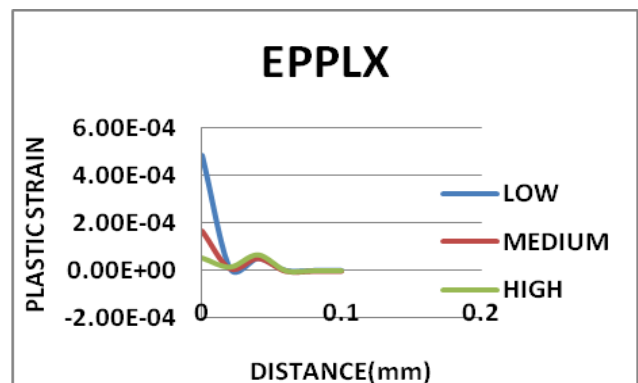
Graph 5.2.3.1 Effect of heat input on plastic strain along X direction
