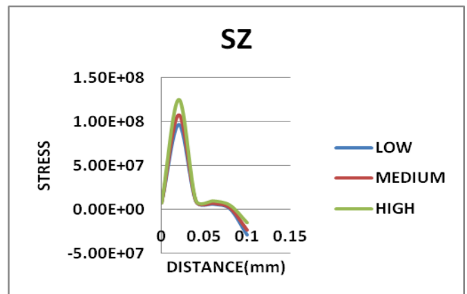
Graph 5.2.4.3 Effect of heat input on stress along Z direction
