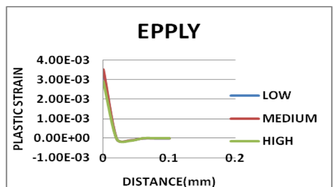
Graph 5.2.3.2 Effect of heat input on plastic strain along Y direction
