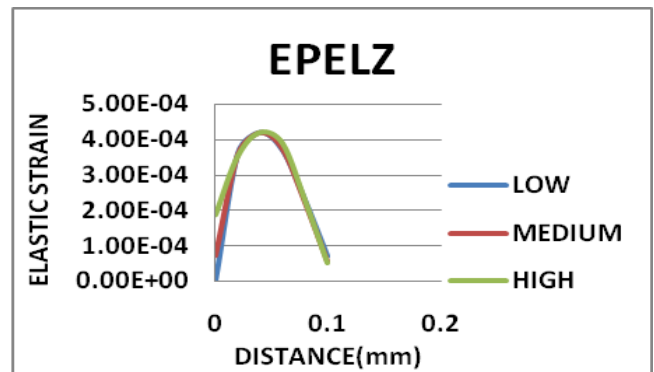
Graph 5.2.2.3 Effect of heat input on elastic strain along Z direction
