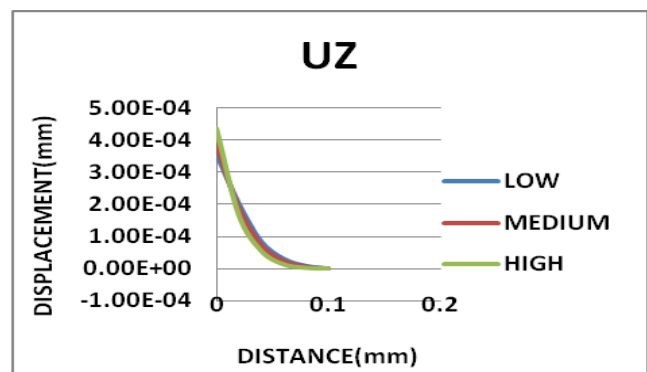
Graph 5.2.1.3 Effect of heat input on displacement along Z direction
