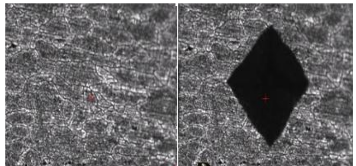
Fig. - 1: A- Position of indenter on the grain before applying the load B- Tested sample after applying the load.
