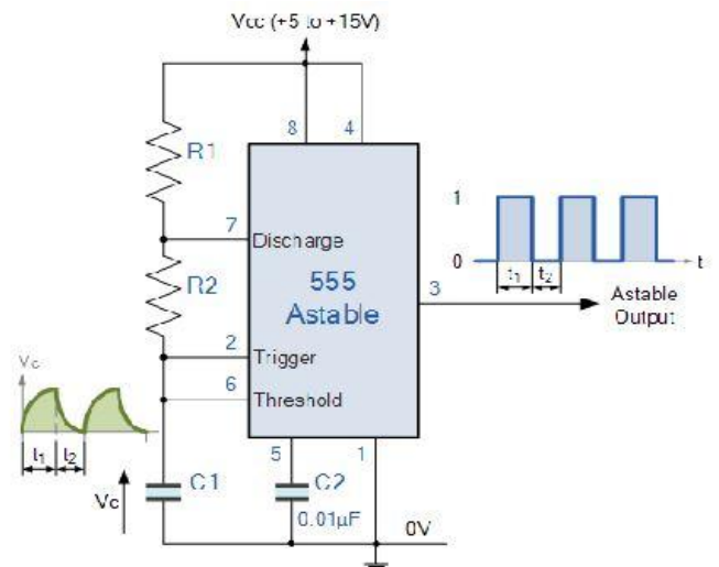
Fig 3: Basic Astable 555 Oscillator Circuit.
