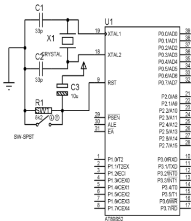
Fig 2: Micro-controller Circuit Diagram.
