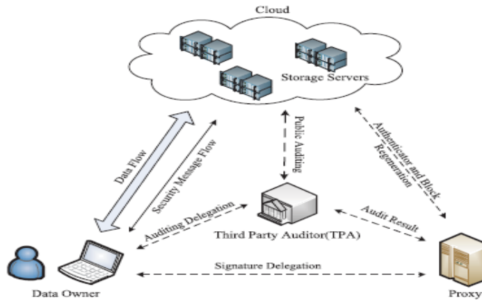
Fig: Cloud Regeneration System Architecture
