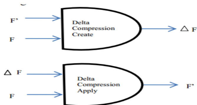
Fig.5: Delta Compression.
