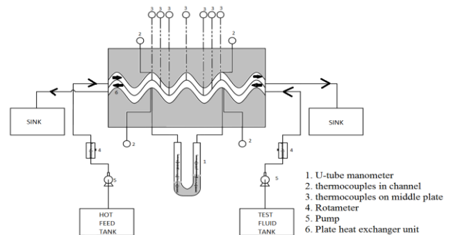
Fig- 1: The experimental setup of corrugated plate heat exchanger.
