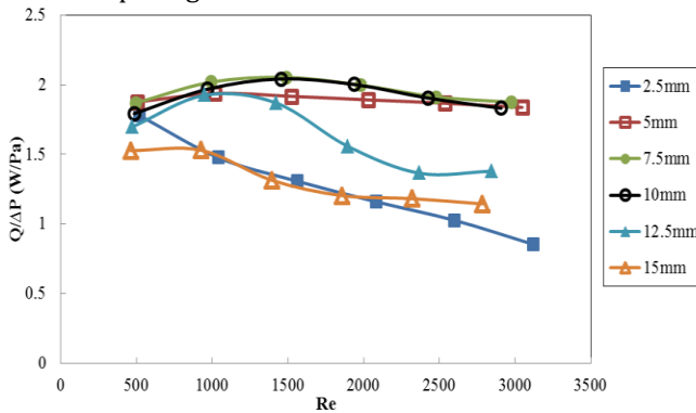
Fig- 10 Comparison of heat transfer rate per pressure drop for various channel spacing's.
