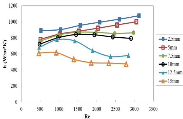
Fig- 8 Comparison of heat transfer coefficient for different cold channel spacing's.
