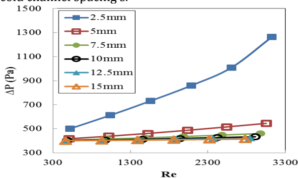
Fig- 9 Comparison of pressure drop for different cold channel spacing's.
