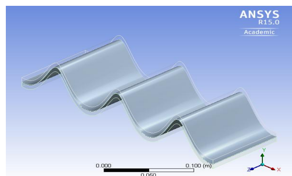
Fig- 2: Geometry created for 30^\circ corrugation angle with 7.5 mm spacing of both hot and cold channel.
