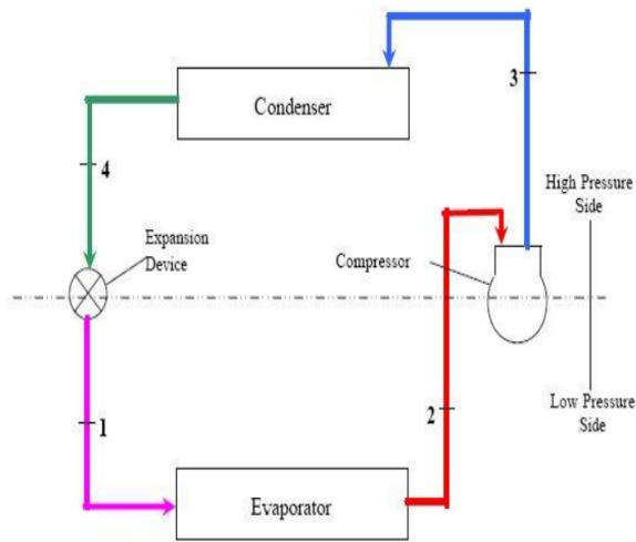
Fig-1: Schematic diagram of simple VCRs
