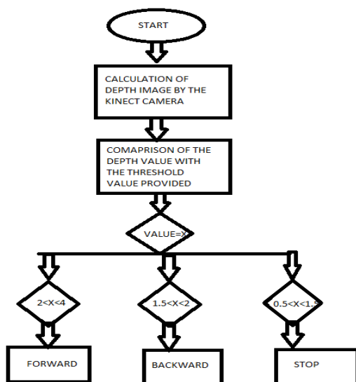
Figure 6 : Overall System Design
