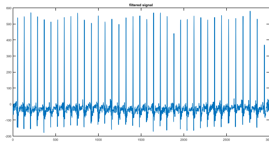
Fig-7: DCT applied ECG signal with noise filtered by Chebyshev Type I filter (low pass) of order 2
