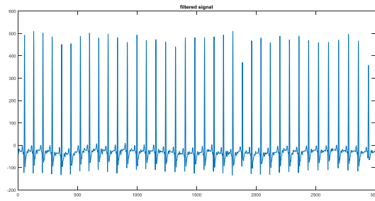
Fig-23: DWT applied ECG signal with noise filtered by Kaiser window of order 10
