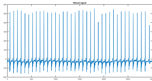
Fig -39: FFT applied ECG signal with noise filtered by Chebyshev filter Type I (low pass) of order 2
