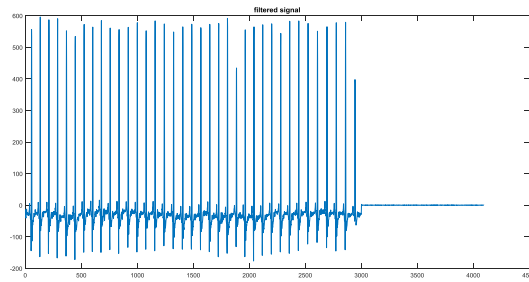
Fig -27: FWHT applied ECG signal with noise filtered by Butterworth filter (low pass) of order 2
