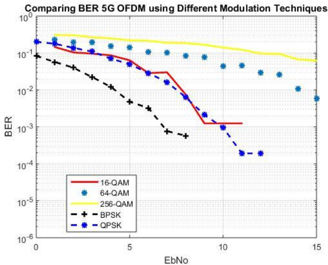
Fig - 5: BER of 5G OFDM for BPSK, QPSK, QAM
