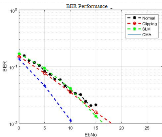
Fig - 6: BER Performance for Normal, Clipping, SLM and CMA PAPR reduction Techniques
