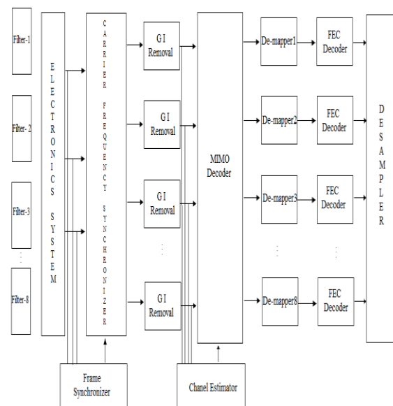
Fig – 2: Block Diagram of the Receiver of IEEE 802.11ac Standard
