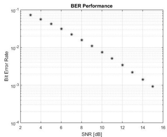
Fig - 3: Bit Error Rate Performance
