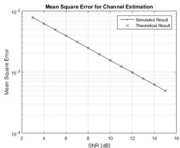
Fig - 4: Mean Square Error for LSE Channel Estimation
