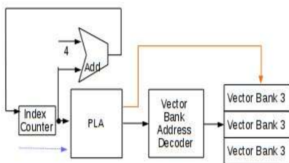
Fig -2: Decoder for Vector bank
