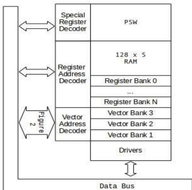
Fig -1: Layout of the RAM with vector register bank
