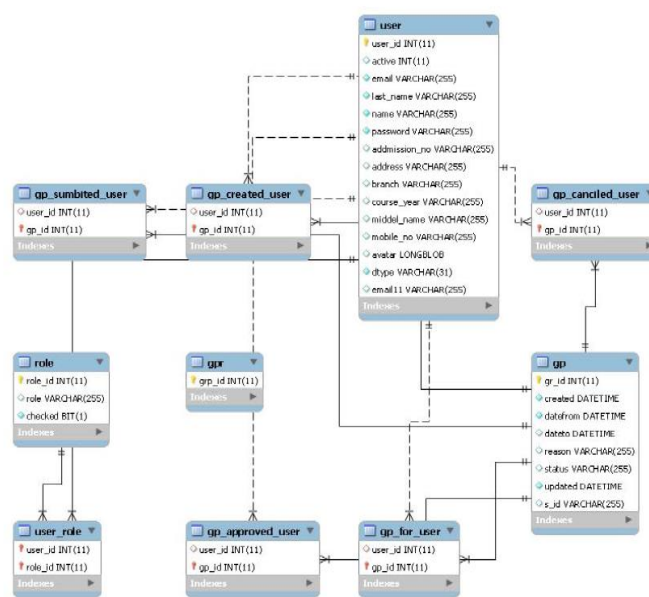
Fig. ER-Diagram of Database
