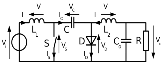
Fig.4 Gird connected PV system with cuk converter
