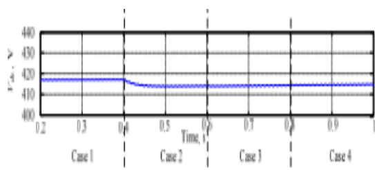
Fig 9.simulation results :Capacitor voltage, V_{dc}
