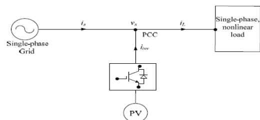
Fig. 1. Block diagram of a grid-connected PV unit
