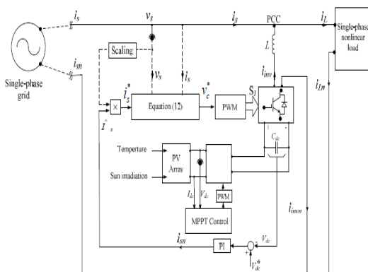
Fig. 7. Block diagram of the proposed control of inverter
