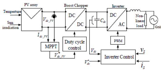
Fig.2. The overall system modelling including control signal
