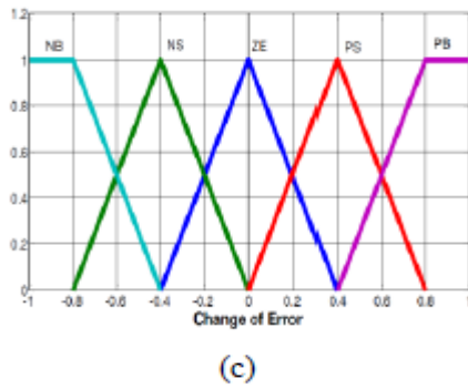
Fig 6, membership function of (a) error E-(b)change of error CE-(c) duty ratio D
