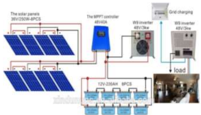
Figure 3: General structure of PV energy.
