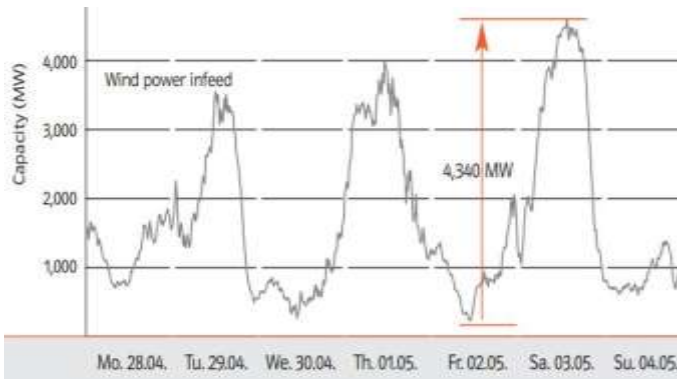
Figure 4: Fluctuations in wind power in E.ON Netz in Germany [1].
