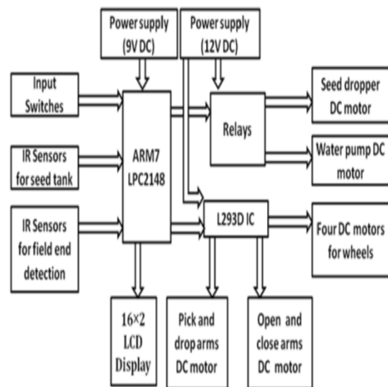
Figure 1. Block diagram
