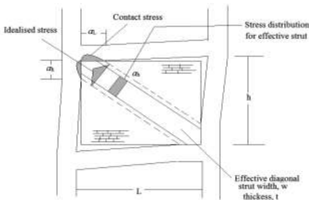
Fig -4: Equivalent diagonal strut
