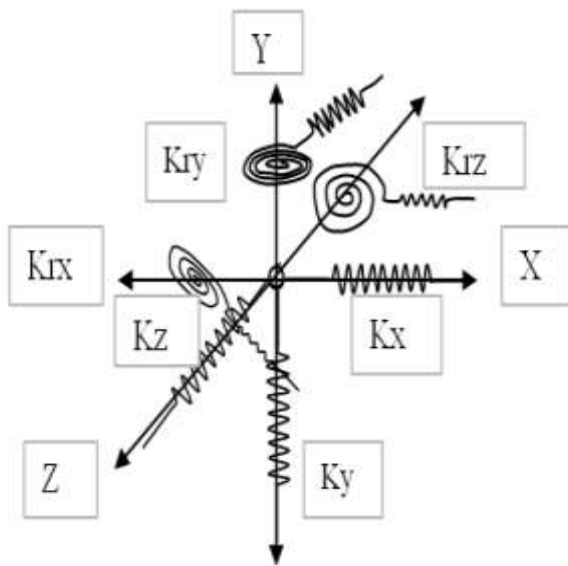
Fig -2: Equivalent soil spring junction
