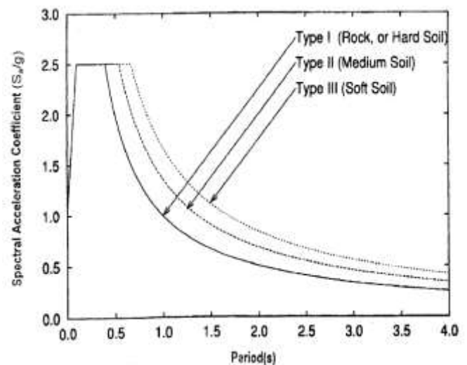
Chart -1: Response spectra for rock and soil sites for 5% damping (IS1893)
