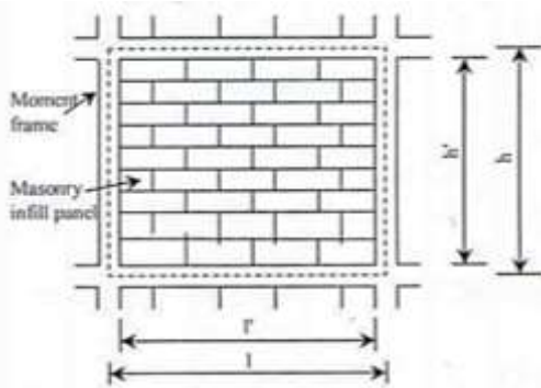
Fig -3: Masonry infill panel in structure Infill wall without opening
