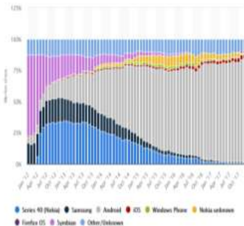
Chart -1: Operating System Usage Distribution [30]
