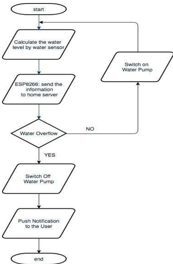
Fig -6: Working of the Water Conservation system
