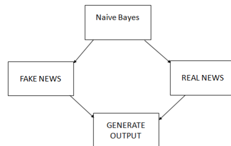
Fig 6.2 Rumor Evaluation
