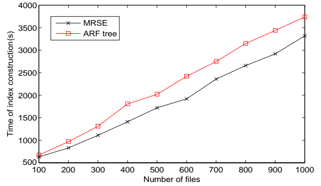
Fig. 12. Construction time of an ARF tree
