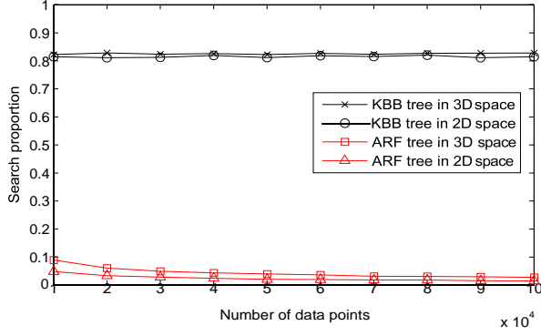
Fig. 7. Search proportion of KBB tree and ARF tree
