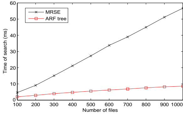
Fig. 13. Search time of a query
