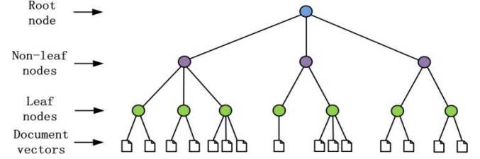
Fig. 6. An ARF tree
