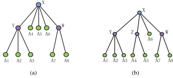
Fig. 3. Examples of access trees.
