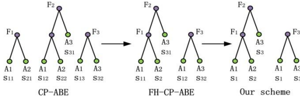
Fig. 5. Comparison of CP-ABE, FH-CP-ABE and our scheme
