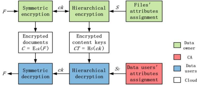
Fig. 4. The flow chart of document encryption and decryption
