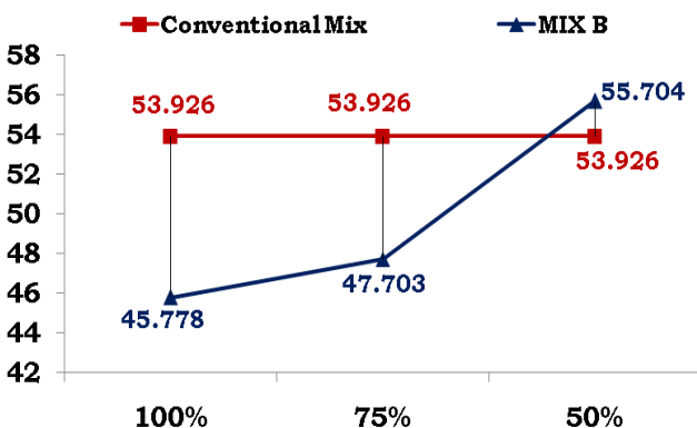
Fig 7: 28 Day's Compressive Strength - Mix B
