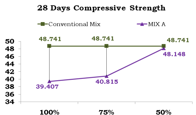
Fig 4: 28 Day's Compressive Strength - Mix A
