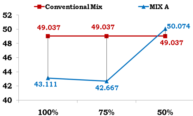
Fig 6: 28 Day's Compressive Strength - Mix A
