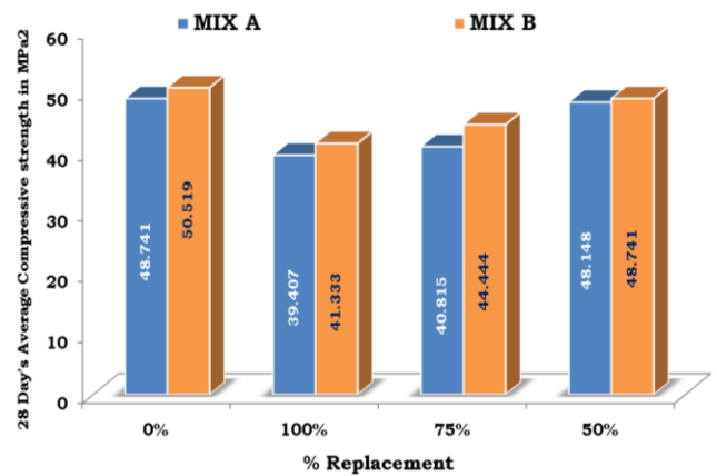
Fig 2: 28 Day's Compressive Strength Graph
