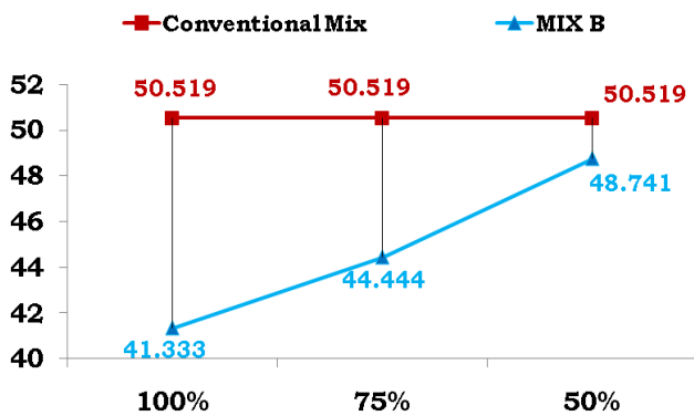
Fig 5: 28 Day's Compressive Strength - Mix B
