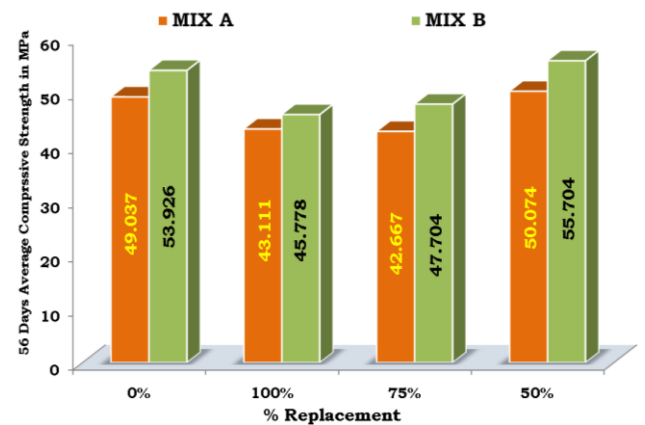
Fig 3: 56 Day's Compressive Strength Graph
