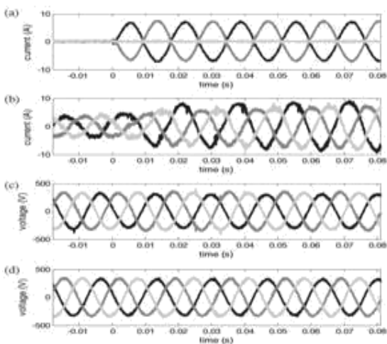
Fig. 9. iUPQC transitory response during the Connection of a two-phase diode rectifier: (a) load currents, (b) source currents, (c) load voltages and Source voltages
