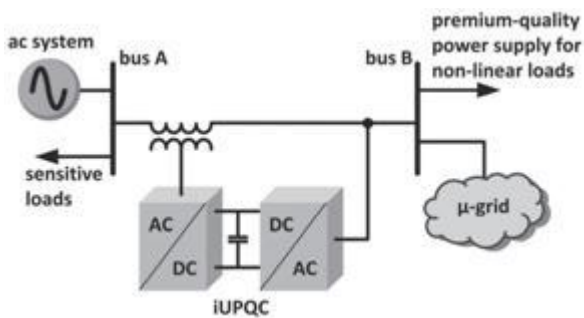
Fig. 1 Example of applicability of iUPQC
