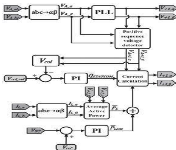
Fig. 2. Novel iUPQC controller.
