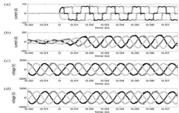
Fig. 8. iUPQC transitory response during the connection of a three-phase diode rectifier: (a) load currents, (b) grid currents, (c) load voltages and (d) grid voltages.
