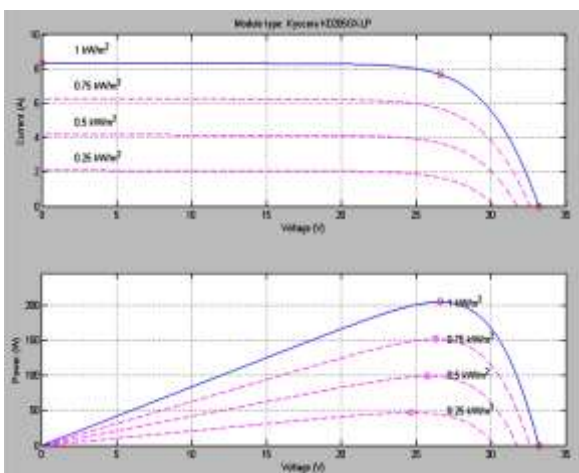
Fig.10: I-V and P-V characteristics of string at 25°C and at different irradiance
