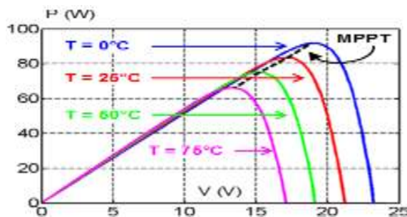
Figure 5 Effect of temperature changes on P-V curves.
