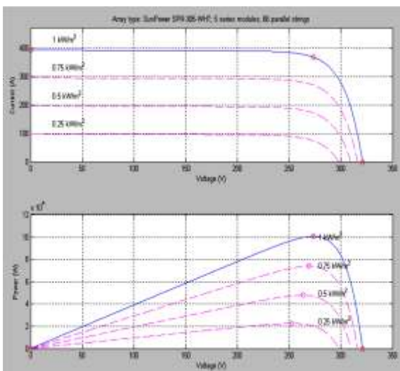
Fig.11: I-V and P-V characteristics of one module at 25°C and at different irradiance
