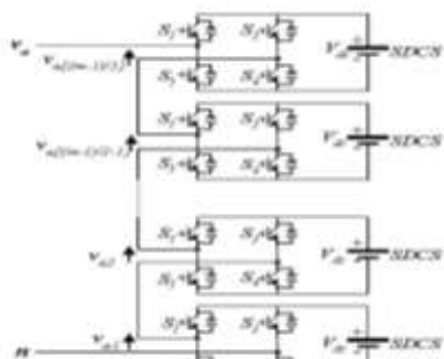
Figure 3 single phase structure of a multilevel cascaded H- bridge inverter.
