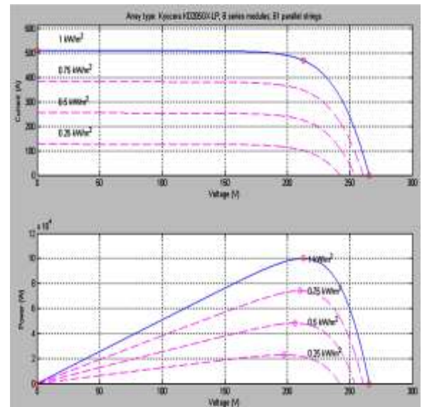
Figure12 I-V and P-V characteristics of string at 25°C and at different irradiance
