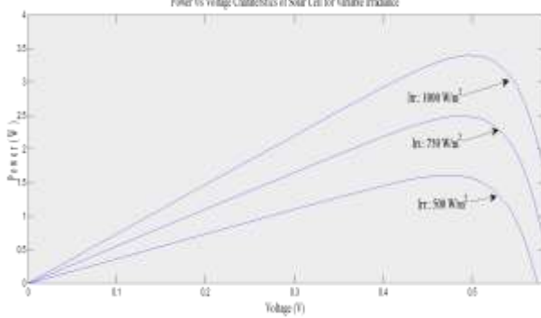
Fig.16: Power v/s voltage characteristic of cell at standard temperature and at different irradiance
