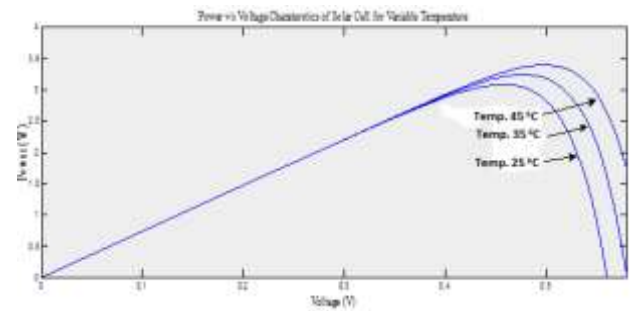
Fig.13: Power v/s Voltage characteristic of PV system at standard irradiance and at different temperature
