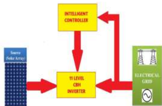
Figure 1 Block Diagram of grid connected PV power system
