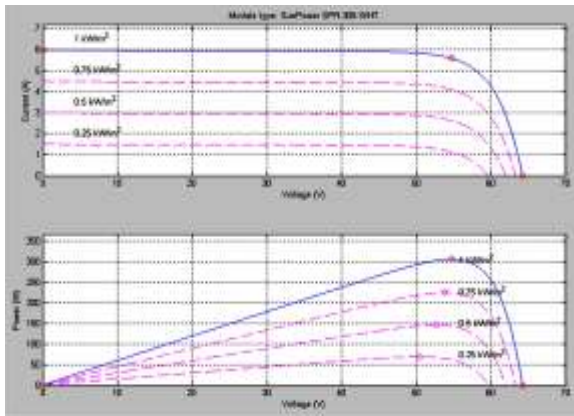
Fig.9: I-V and P-V characteristics of one module at 25°C and at different irradiance
