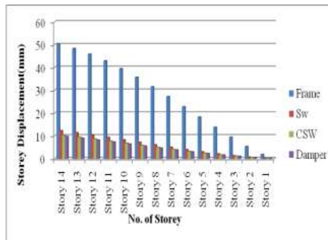
Fig 6.2 Storey displacement in y direction due to EQY
