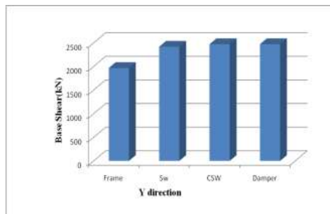
Fig 6.1 Base shear in y direction due to EQY
