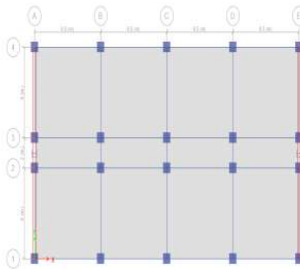
Fig. 5.1 Plan of G+13 storey building
