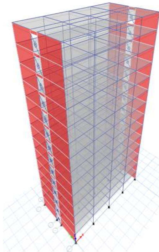
Fig. 5.2 3D view of G+13 storey building
