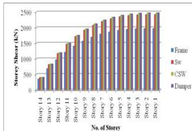
Fig 6.5 Storey shear in y direction due to EQY
