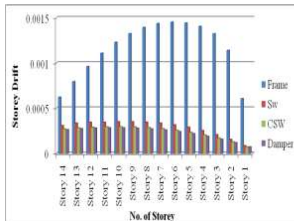
Fig 6.4 Storey drifts in y direction due to EQY
