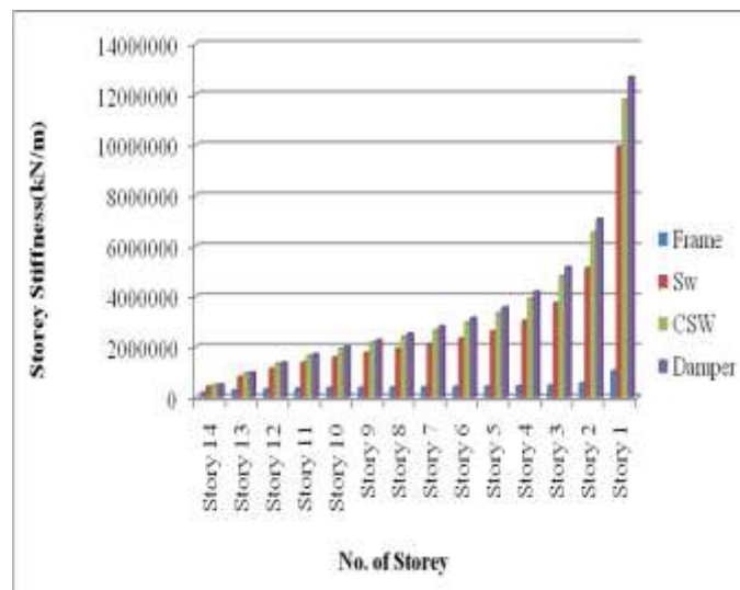
Fig 6.3 Storey stiffness in y direction due to EQY
