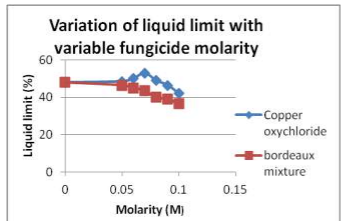
Chart -1: Variation of Liquid limit with fungicide addition
