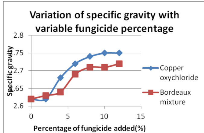
Chart -3: Variation of Specific gravity with fungicide addition
