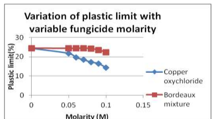
Chart -2: Variation of Plastic limit with fungicide addition
