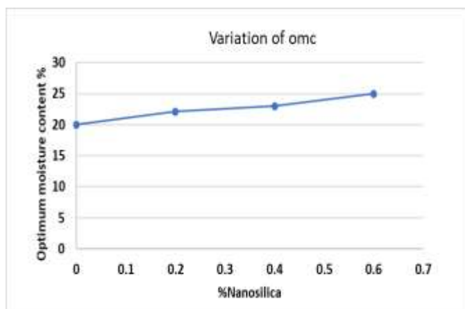
Chart 1 Variation on OMC with different percentages of Nanosilica.
