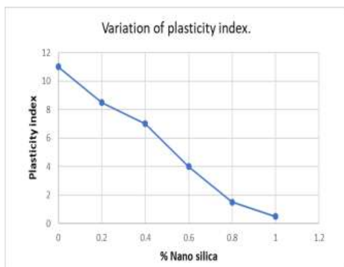
Chart 5 . Variation of plasticity index with the addition of Nano silica.
