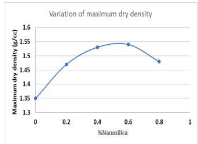
Chart 2 Variation on MDD with different percentages of Nanosilica.
