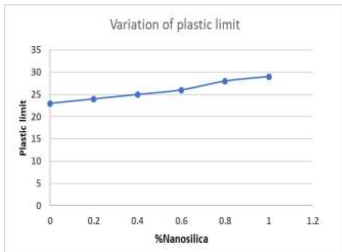
Chart 4 Variation of plastic limit with the addition of Nano silica.
