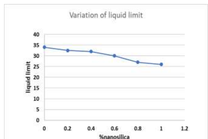
Chart 3 . Variation of liquid limit with the addition of Nano silica.
