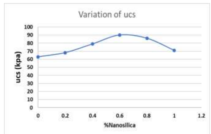
Chart 6 Variation of UCS with Nano silica.
