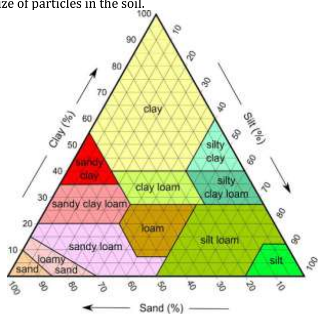
Fig-1: Soil textural classification
