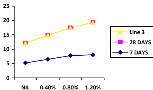
Chart-3: Flexural strength
