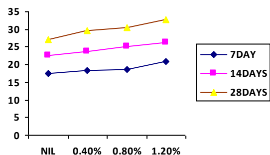
Chart -1: Compressive strength
