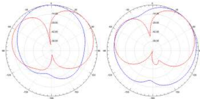
Fig. 7 E-Field and H-Field Radiation pattern at 4.05GHz (Red: \theta=0^\circ , Blue: \Phi=90^\circ )
