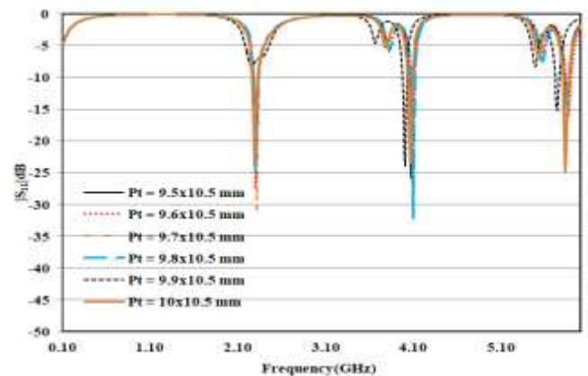
Fig 5: Return loss of antenna for variation fed position
