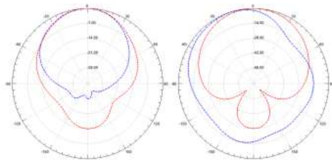
Fig. 8 E-Field and H-Field Radiation pattern at 5.85 GHz (Red: \theta=0^\circ , Blue: \Phi=90^\circ )
