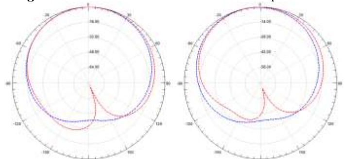
Fig 6: E-Field and H-Field Radiation pattern at 2.3GHz (Red: \theta=0^\circ , Blue: \Phi=90^\circ )
