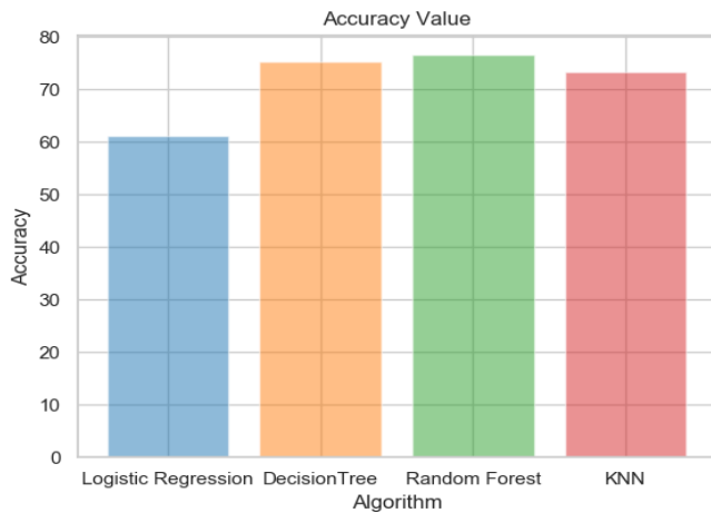
Fig-1: Comparison Analysis of the Machine Learning Algorithms
