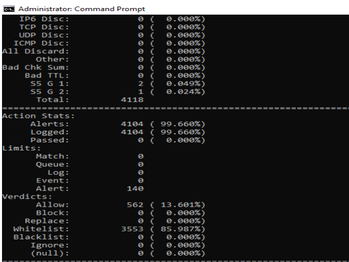
Fig-2: Alert Checking in Snort
