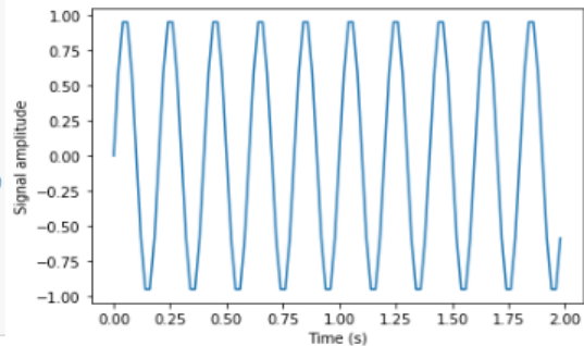
Fig -6: Depiction of Wave using DFT
