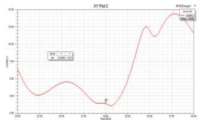
Fig. 8 VSWR plot of 2x2 array antenna with slot
