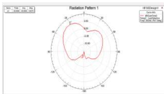
Fig. 5 Gain pattern of 2x2 array antenna without slot
