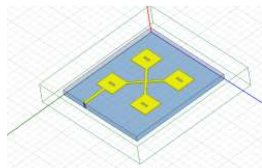
Fig. 2 Geometry structure of 2x2 array antenna with slot
