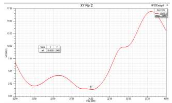
Fig. 7 VSWR plot of 2x2 array antenna without slot
