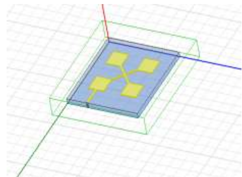
Fig. 1 Geometry structure of 2x2 array antenna without slot
