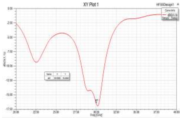
Fig. 3 S11 (in dB) of 2x2 array antenna without slot
