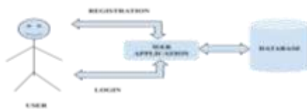
FIG.2 USER REGISTRATION
