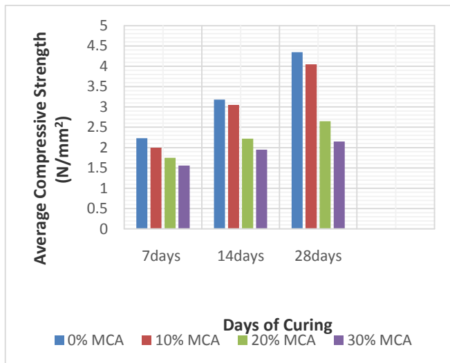
Fig -1: Average Compressive Strengths of Blocks
