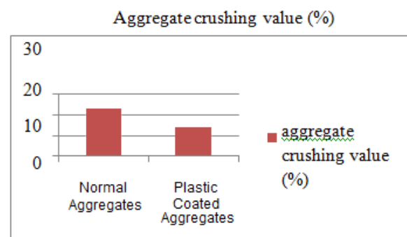
Figure 1 – Aggregate crushing value
