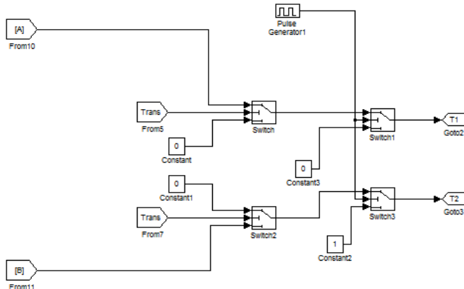
fig-6 forward motoring triggering logic
