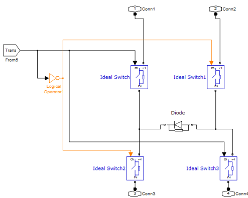
Fig-5 sub circuit of reversible FWD (right)
