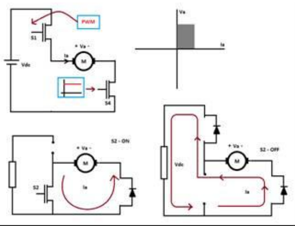
Fig-2 Schematic showing type of triggering in quadrant 1 (top left), first quadrant representation (top right), Braking mode with s2 closed (bottom left), Braking mode with s2 opened (bottom right)
