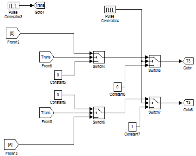
Fig-7 Reverse motoring Triggering logic
