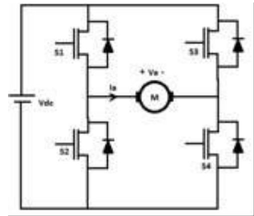
Fig1 Class E Chopper diagram
