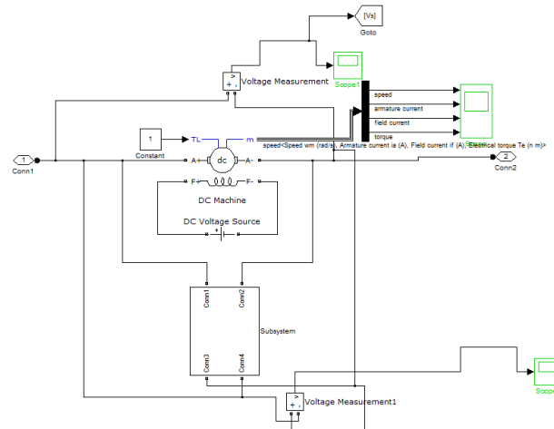
fig-4 sub circuit of reversible fwd (left)
