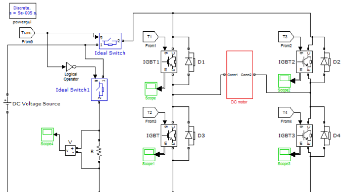
Fig-3 Simulink model of proposed model
