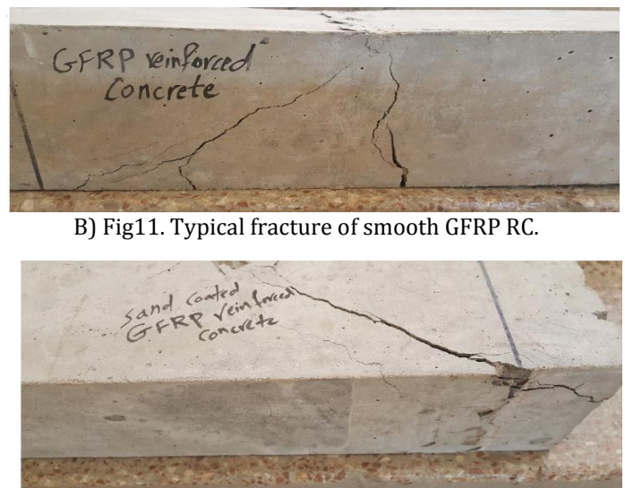
C) Fig 12. Typical fracture of sand coated GFRP RC.
