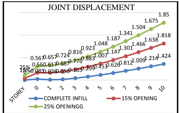
Graph: Displacement
