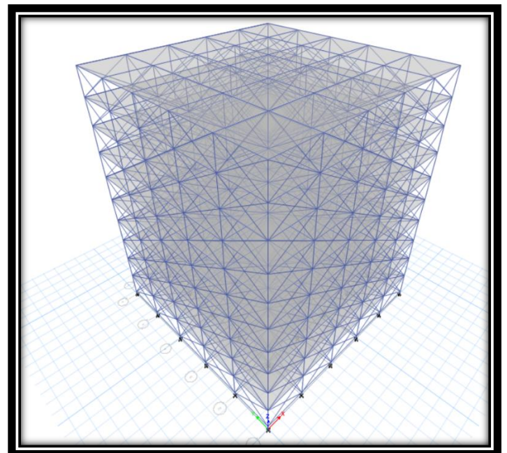
Fig. Diagonal Strut
