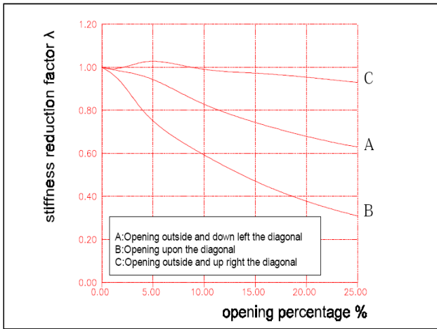
Fig. (A)Frame with Opening (B)Stiffness reduction factor λ' of the infilled frame in relation to the opening percentage (a,b,c)
