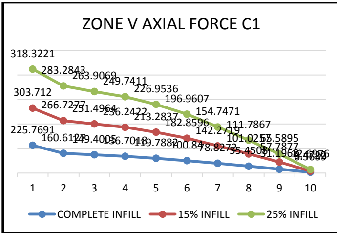
Graph: AXIAL FORCE
