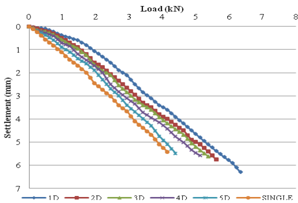
Fig. 2 Load settlement behavior of interfering circular footings
