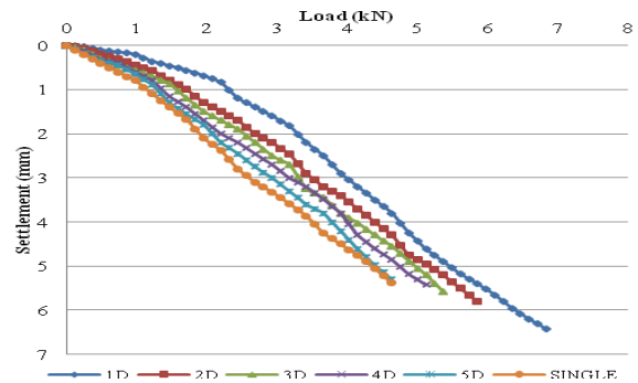
Fig. 3 Load settlement behavior of interfering ring footings
