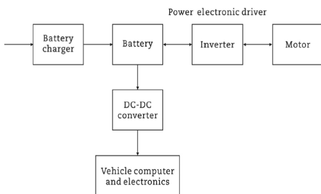
Fig-1: Key component of an electric vehicle
