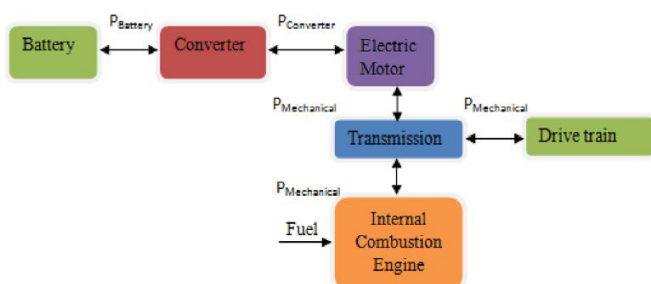
Fig -3: Power Flow of Hybrid EV
