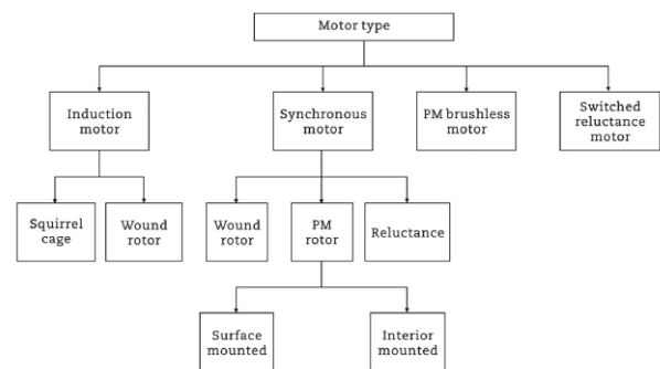
Fig -2: Various Motors Used In Electrical Vehicle
