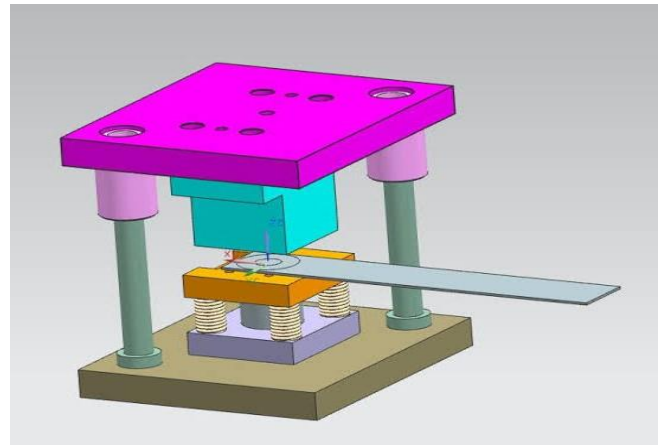
Fig - 3: 3 D View of compound Die [Example]
