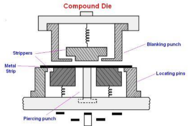
Fig - 1: Compound Die
