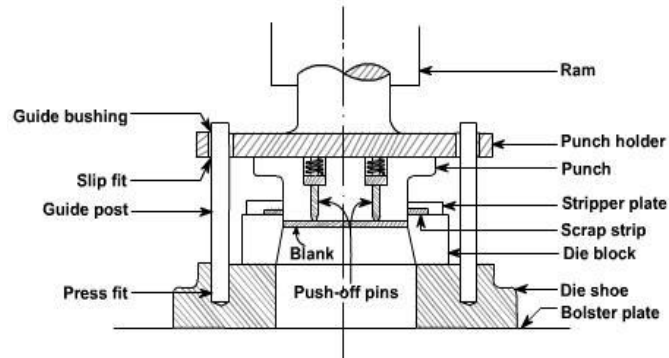
Fig - 2: Basics of blanking tool
