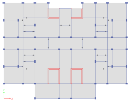
Fig -4: Architectural Plan of the Structure for all different sloped grounds
