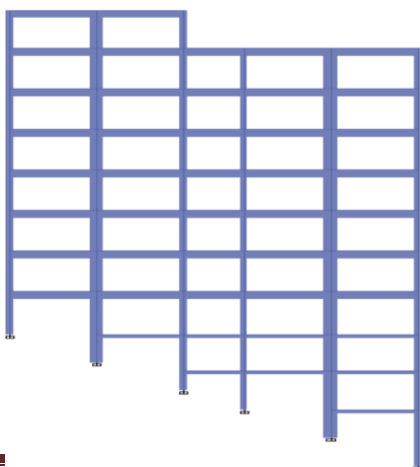
Fig -7: Structure with 20 degree slope
